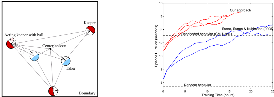
Figure 1: Left: Illustrating keepaway . The various lines and angles indicate the 13 state variables making up each sensation. Right: Learning curves for our approach. We plot training time (after interacting for 20 hours an agent experiences roughly 50,000 state transitions) against the average time the keepers are able to control the ball (quality of learned behavior).
